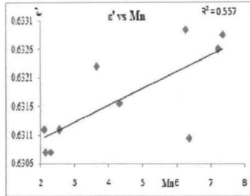
Figure 14: variation of dielectric constant with manganese in soil
