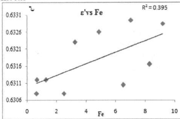
Figure 13: variation of dielectric constant with iron in soil
