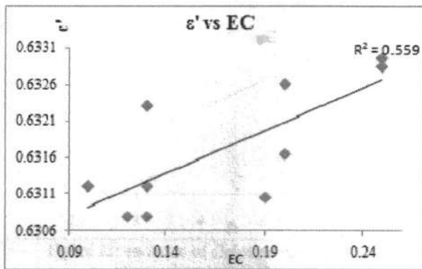
Figure7: variation of dielectric constant with electrical conductivity of soil
