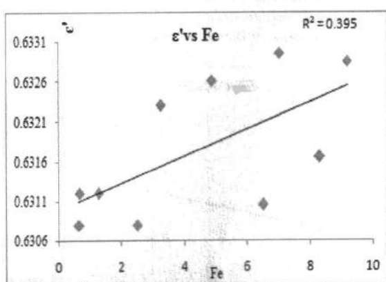
Figure 13: variation of dielectric constant with iron in soil
