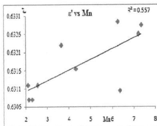
Figure 14: variation of dielectric constant with manganese in soil
