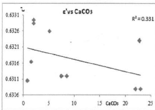
Figure 9: variation of dielectric constant with calcium carbonate in soil
