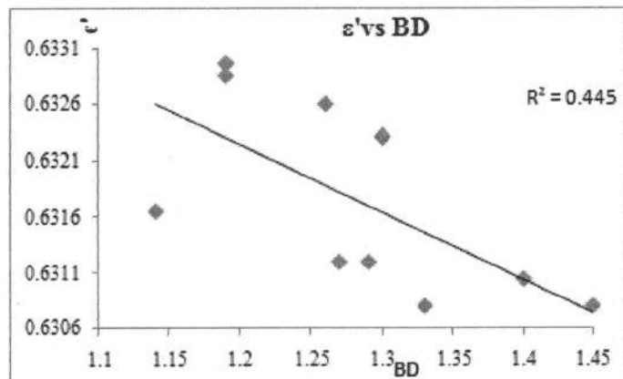
Figure 4: variation of dielectric constant with bulk density of soil
