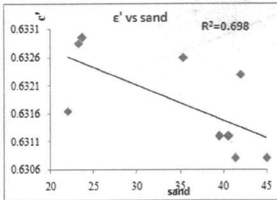
Figure 1: variation of dielectric constant with % of sand in soil
