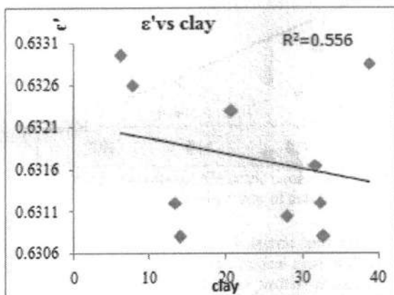
Figure 3: variation of dielectric constant with % of clay in soil
