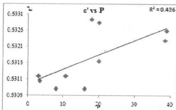
Figure 11: variation of dielectric constant with phosphorous in soil
