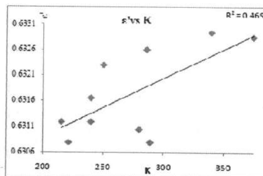
Figure 12: variation of dielectric constant with potassium in soil
