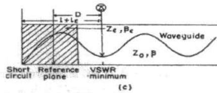
Fig 2 Illustration of Wave-Guide Cell Method for measuring dielectric constant [a]. Double minimum width [b]. Position of minimum with shorted waveguide without dielectric [c]. Position of minimum with shorted waveguide with dielectric sample.
