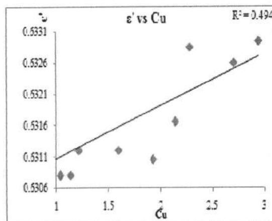
Figure 16: variation of dielectric constant with copper in soil
