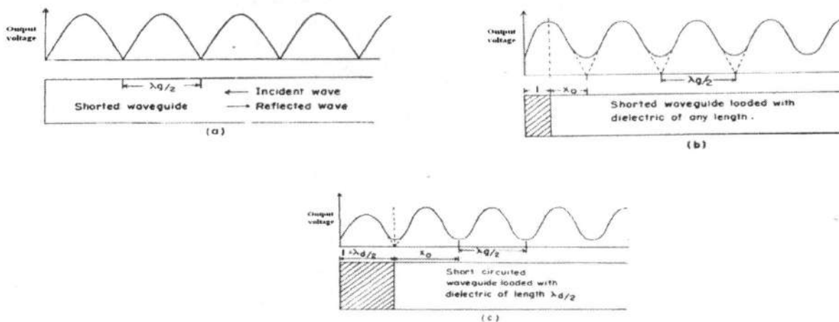
Fig.1 Standing Waves in a waveguide [a]. without dielectric [b]. loaded with dielectric of any length [c]. loaded with dielectric of length \lambda_d/2 [ \lambda_d is the wavelength of microwaves in the dielectric].
