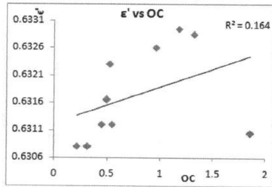
Figure 8: variation of dielectric constant with organic carbon in soil
