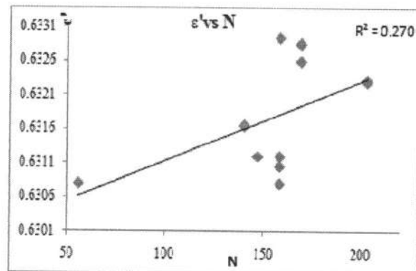
Figure 10: variation of dielectric constant with nitrogen in soil
