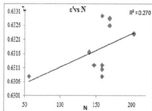
Figure 10: variation of dielectric constant with nitrogen in soil
