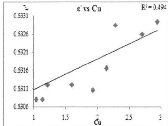
Figure 16: variation of dielectric constant with copper in soil
