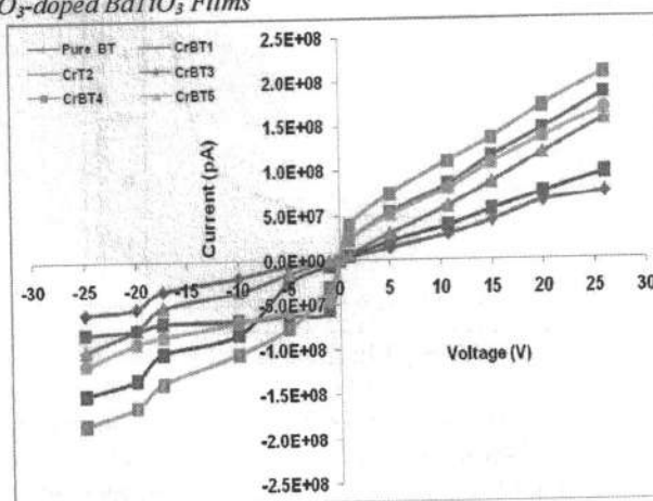
Fig. 3 I-V characteristic for pure BT, CrBT1, CrBT2, CrBT3, CrBT4 and CrBT5
