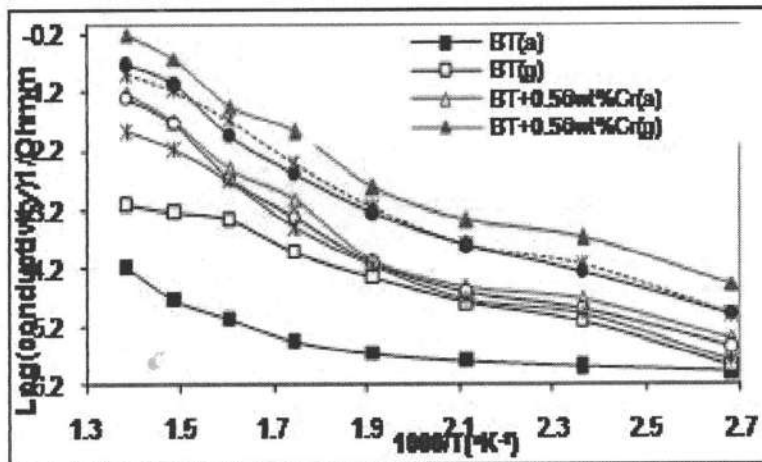
Figure 4 : Variation of electrical conductivity with temperature.
