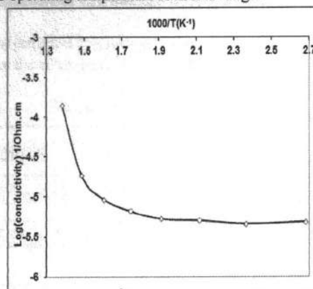
Fig. 5: Variation of conductivity with temperature
